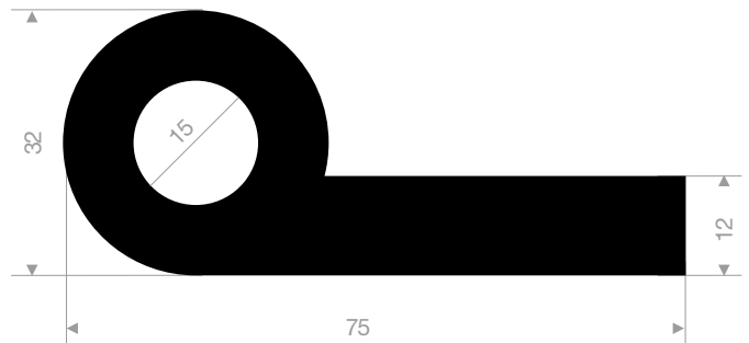
VR21400866 EPDM 70° Shore black roll length 20 meter
