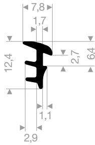
VR21603545 EPDM 65° Shore black roll length 200 meter
