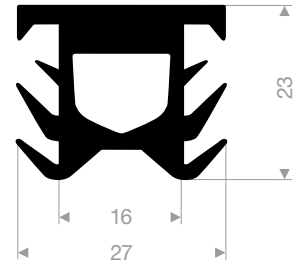
VR21605277 EPDM 70° Shore black roll length 25 meter
