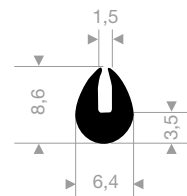
VR21100018 EPDM 70° Shore black roll length 100 meter
