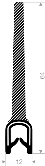
VR24500865 pvc + sponge rubber clamping range 1-2,5 mm roll length 50 meter
