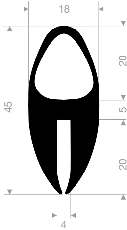
VR21109004 EPDM 65° Shore black roll length 50 meter
