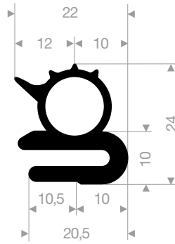
VR21109118 NBR 65° Shore black roll length 25 meter
