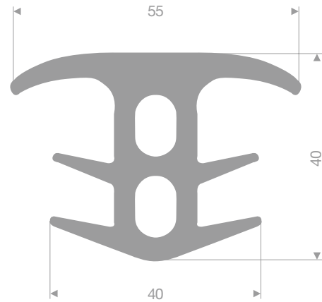
VR21605801GR EPDM 70° Shore grey roll length 15 meter
