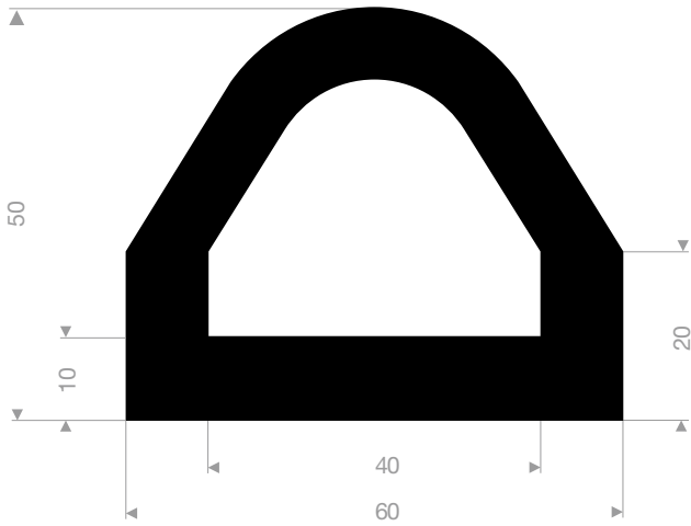
VR21506050 EPDM 70° Shore black roll length 5 meter
