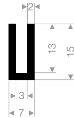
VR21100435 EPDM 70° Shore black roll length 100 meter
